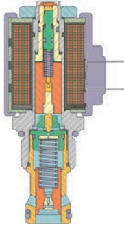
Cartridge valve cutaway
